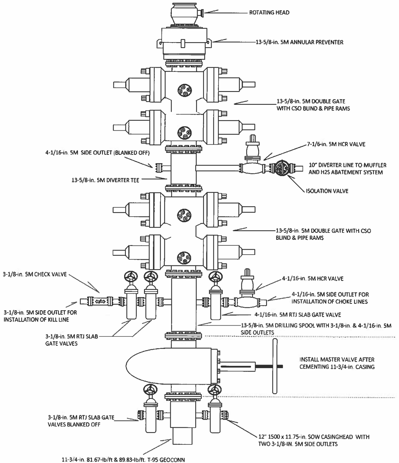
Figure 5. BOP for 11-3/4-inch casing while drilling 9-7/8-inch hole.
