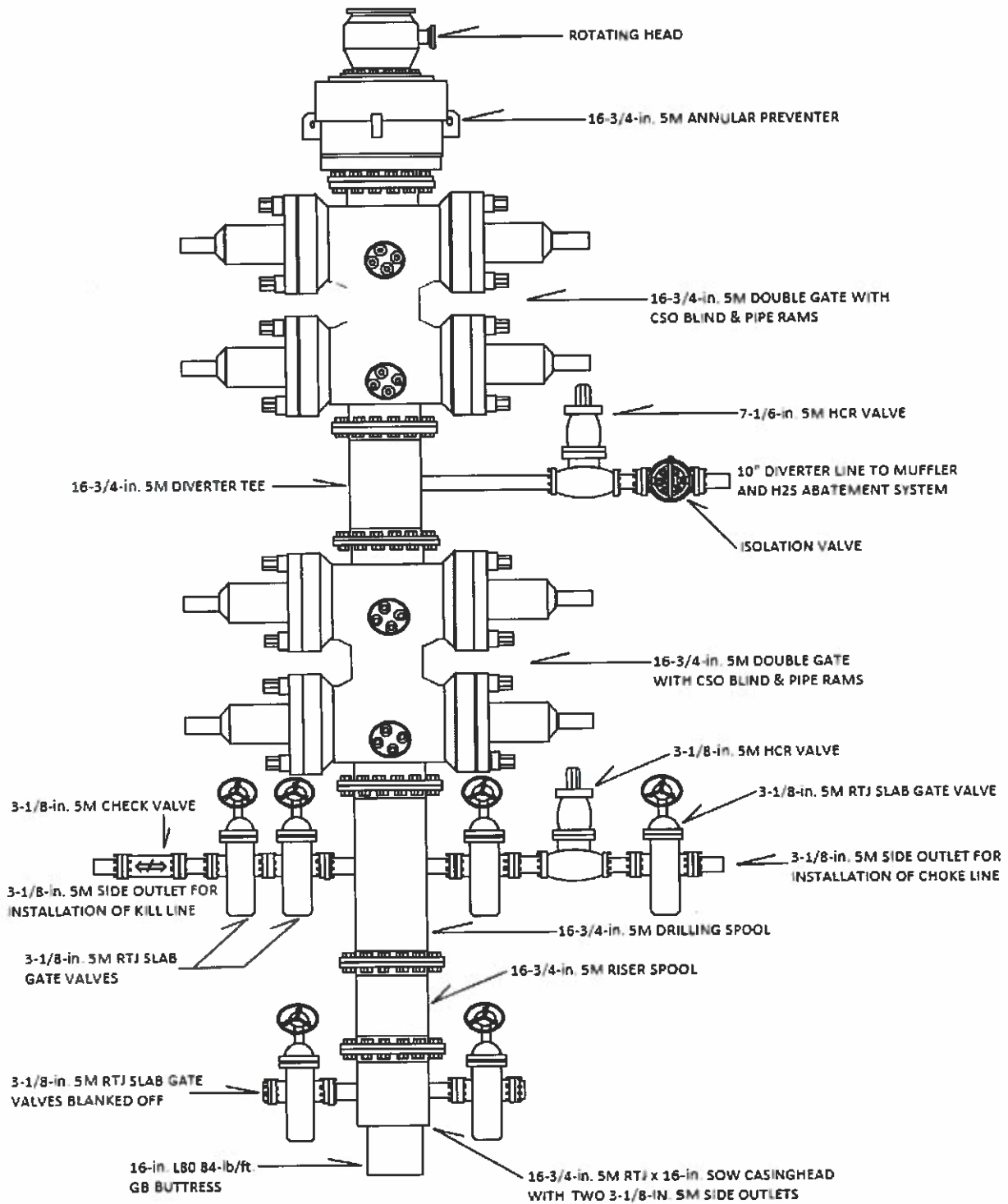
Figure 4. BOP for 16-inch casing while drilling 14-3/4-inch hole.
