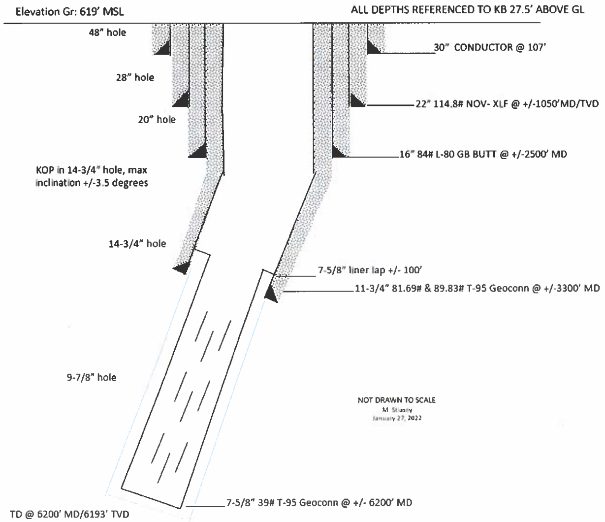
Figure 2. Well Construction Schematic
