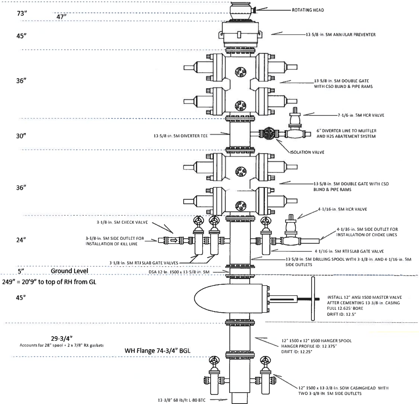
Figure 3. 13-5/8-inch 5M BOPE for 13-3/8-inch casing while drilling 12-1/4-inch hole.
