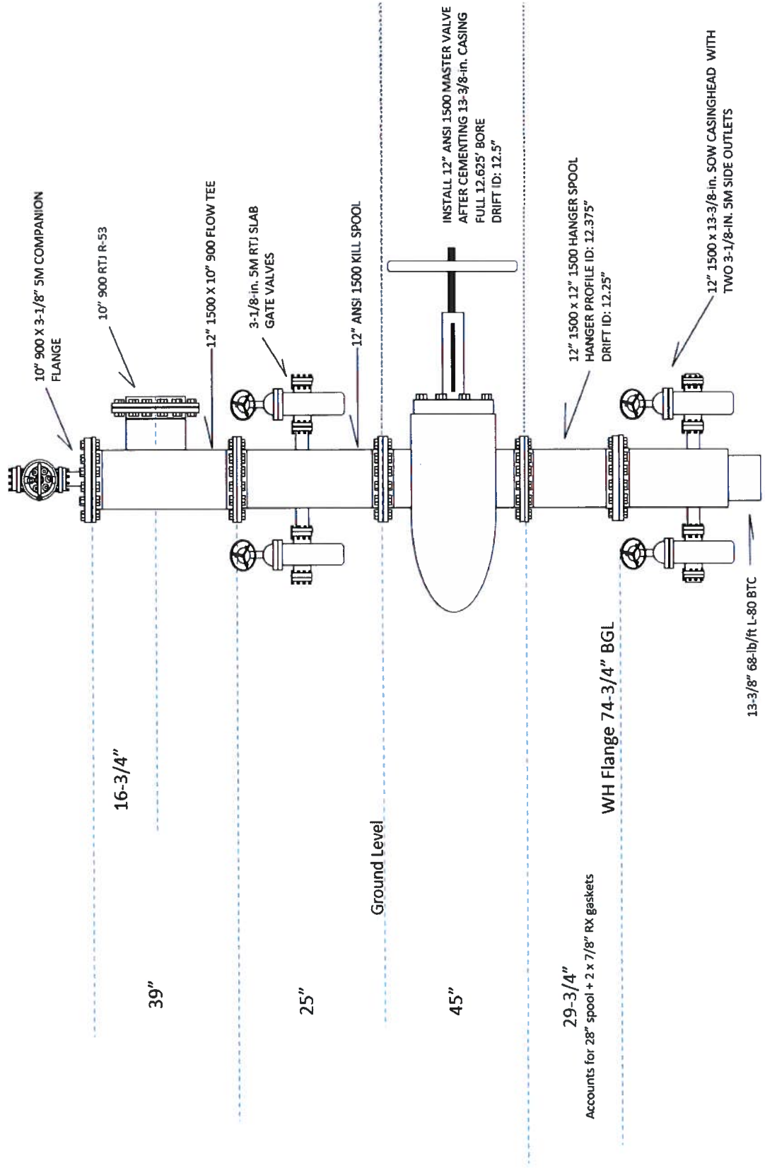
Figure 4. Proposed KS-21 wellhead assembly
