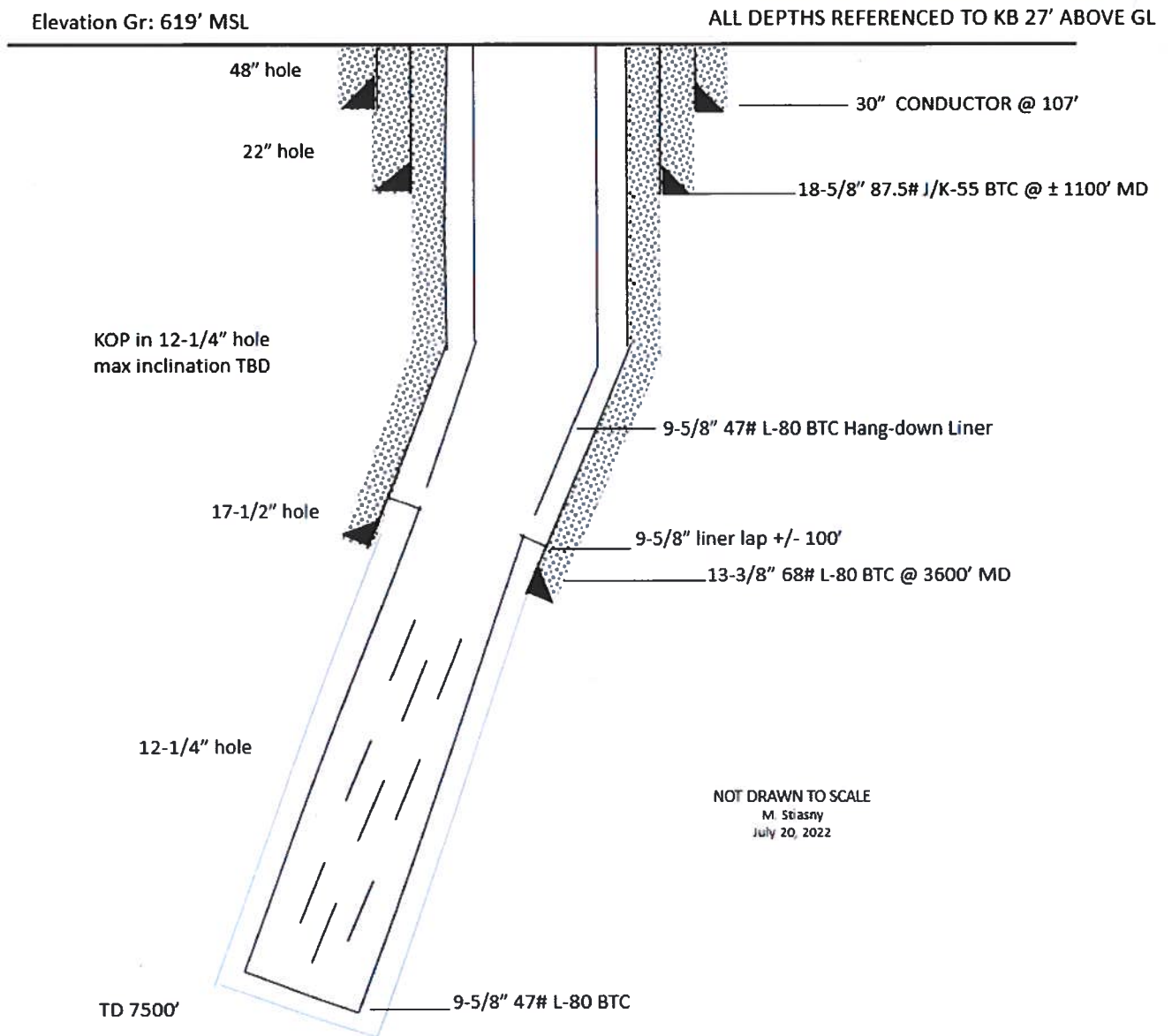
Figure 2. Primary Well Construction Schematic
